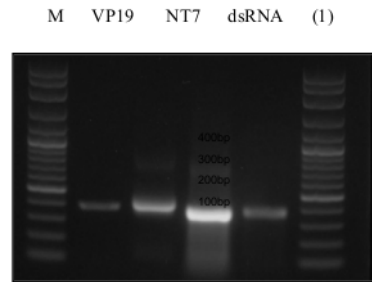
Gambar 2. Electrophoresis produced by WSSV dsRNA-VP19. M = marker100 +, VP19 = VP19 gene, NT7 = nexted promoter T7, dsRNA = WSSV dsRNA-VP19 production.
